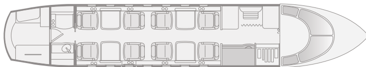
EIGHT-SEAT STANDARD ARRANGEMENT
